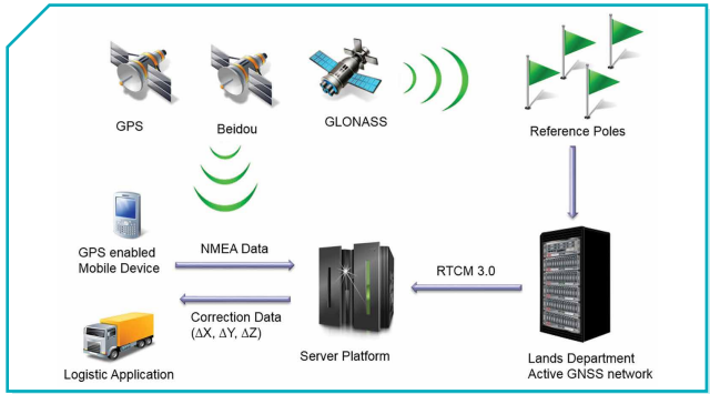
Development of a Hong Kong Positioning Infrastructure Based on GPS, Beidou, and Ground Based Augmentation System 基於GPS、北斗及地面增強系統的香港衛星定位平台
