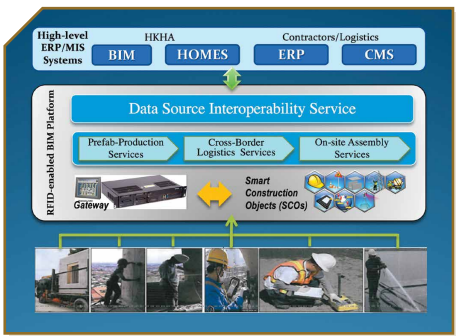
RFID-Enabled BIM Platform for Prefabrication Housing Production in Hong Kong 基於RFID的香港預製房屋建設訊息平台
