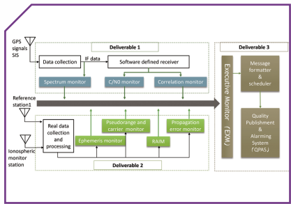
Hong Kong GNSS Signal Quality Monitoring and Interference Detection System GNSS質量監測與干擾檢測系統
